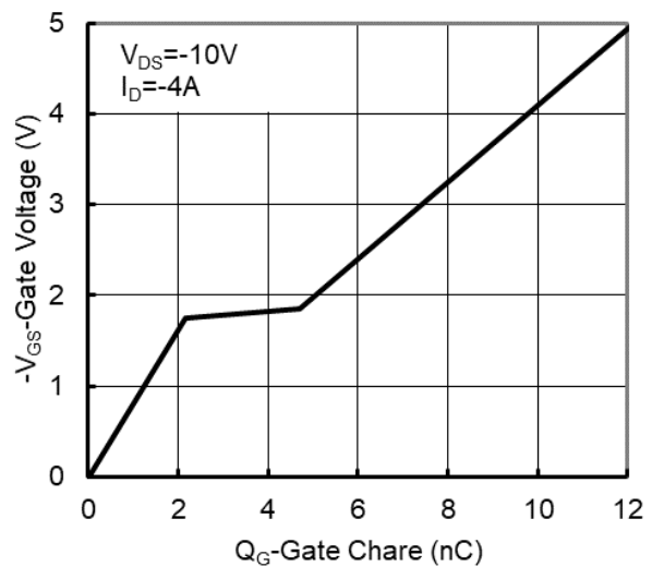
Figure6. Gate Charge
