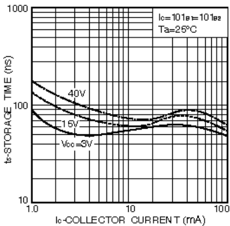
Fig. 10 Storage time vs. collector current
